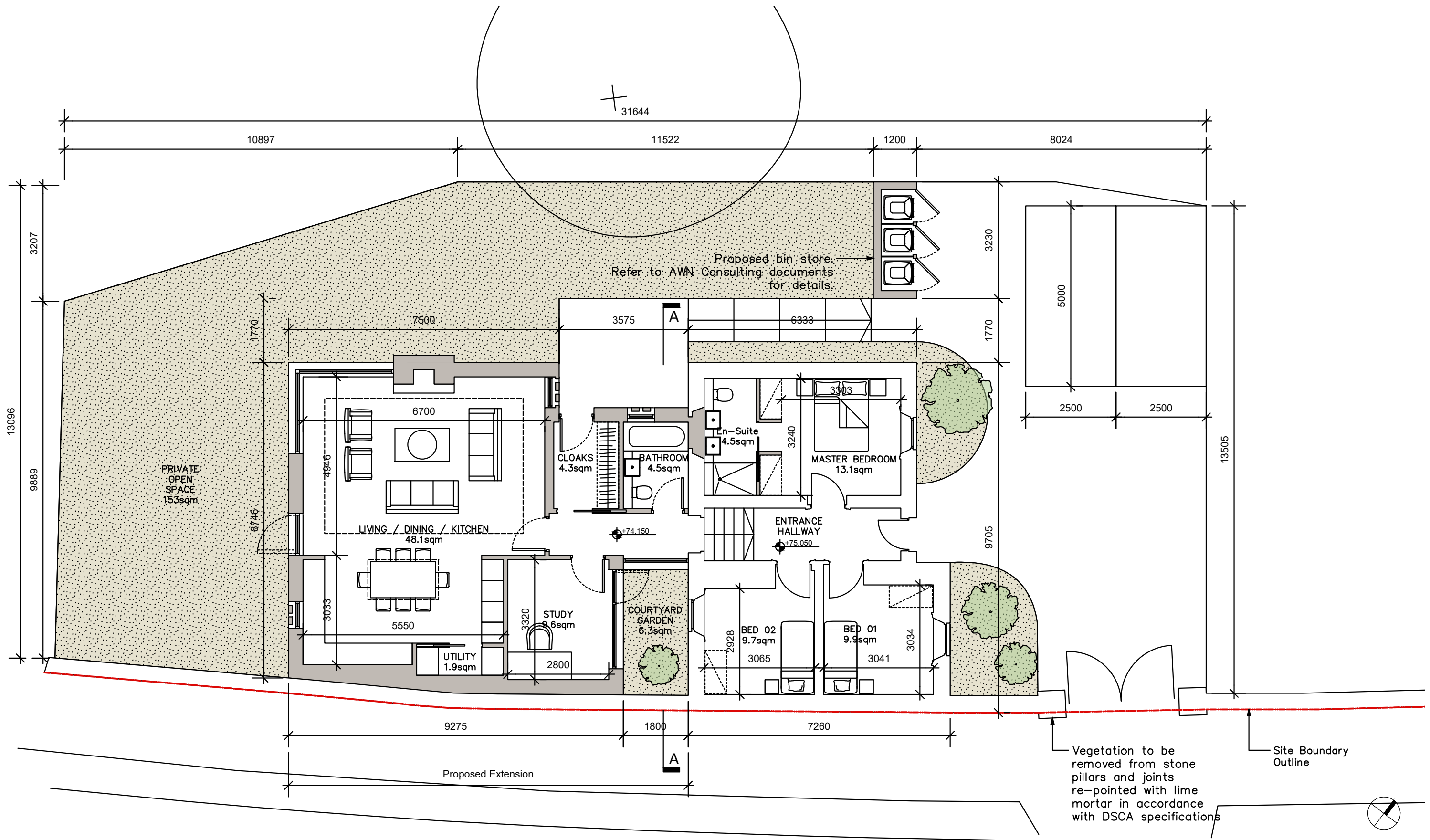
Gate Lodge, Proposed Ground Floor Plans
